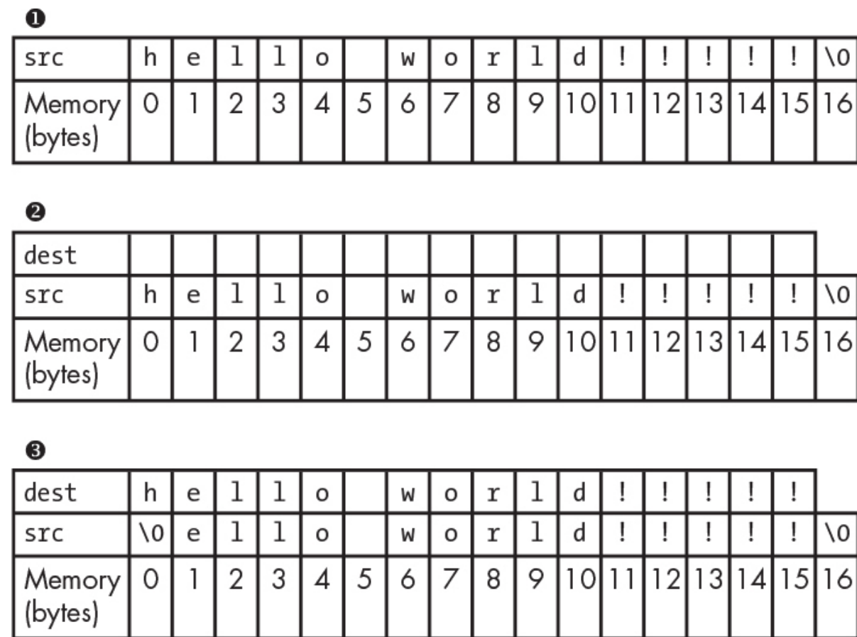
Figure 13-1: How memory overflows from dest to src
